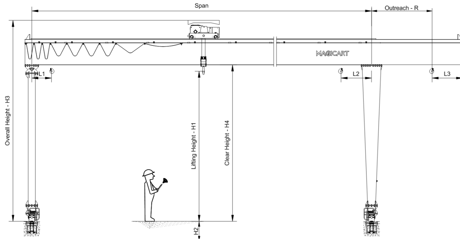
CRANE LAYOUT
